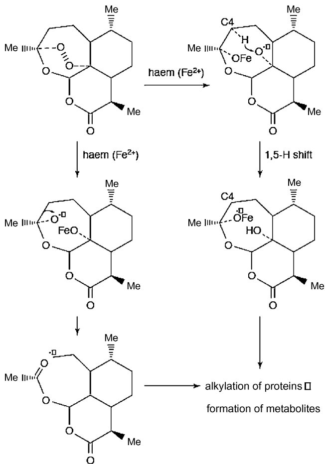
Fig. 3. One of the proposed mechanisms of action. Upon reduction of the peroxide bridge by \text{Fe}^{2+} , two radical anions can be formed. In one of these a 1,5-H shift between the oxygen radical and a hydrogen atom at C4 occurs with formation of a carbon radical and subsequent formation of a presumed epoxide intermediate which is electrophilic and can react with proteins. Rearrangement of the other oxygen radical intermediate gives rise to a primary radical involved in the alkylation of haem and parasite proteins leading to parasite death (van Agtmael et al., 1999).
